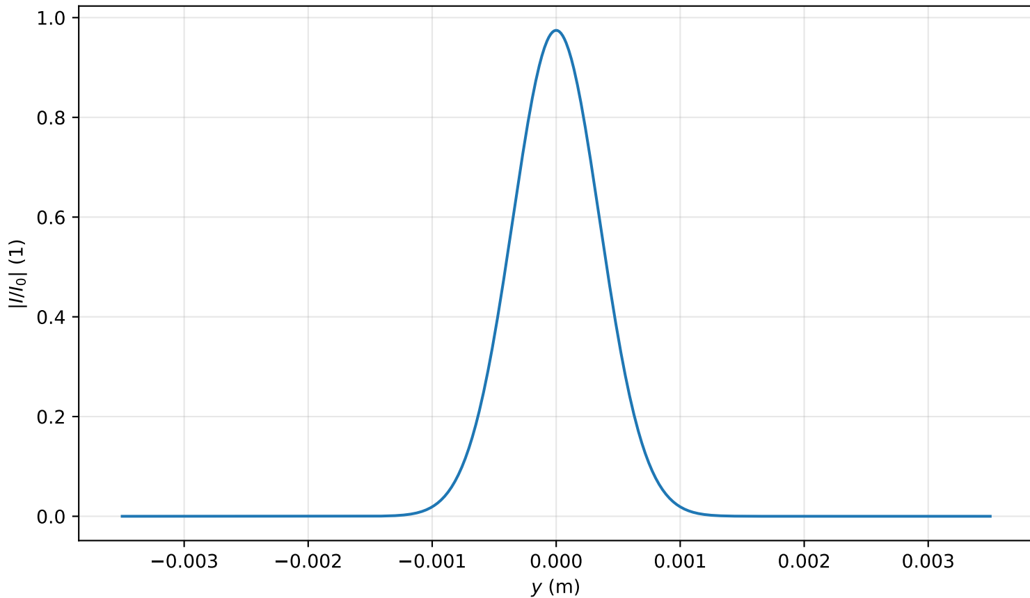
Intensity profile I(x=0, y, z=0.398)/I_0 , \text{Pin}=0.1\text{Pcr} , artificial time
